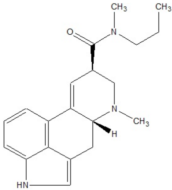
Lysergic acid methylpropylamide
