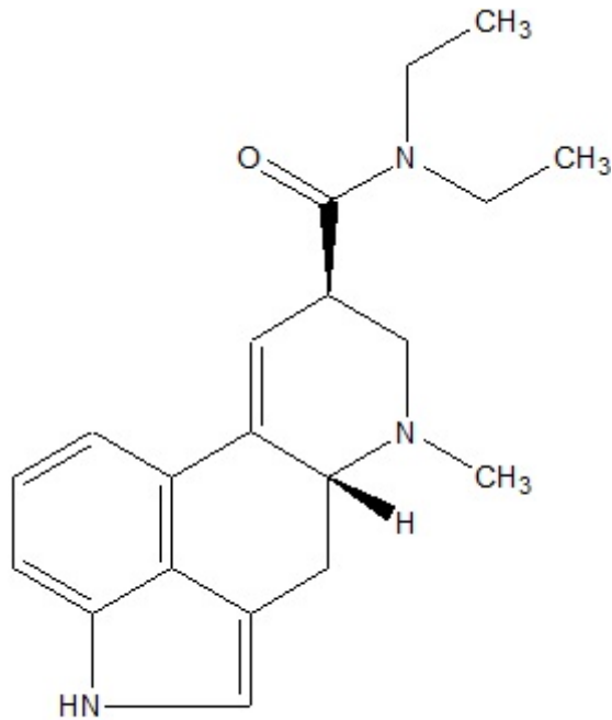
Lysergic acid diethylamide
